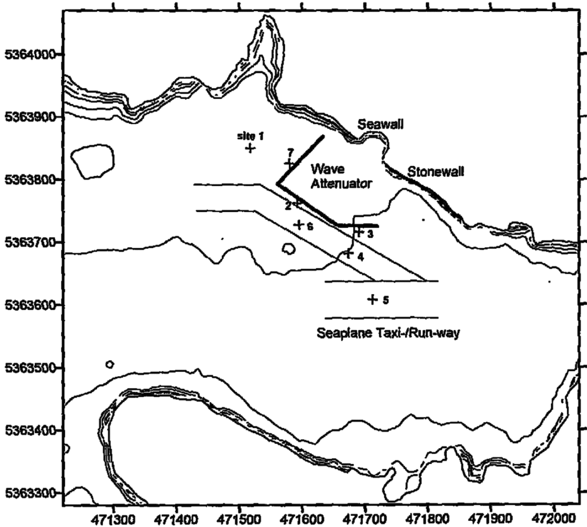
Figure 1: A map showing the new design of the VIM attenuator (the heavy red line) and the locations of the SWAN model output in the form 3D Wave Spectra. Sites 2, 3 and 7 are immediately alongside the Marina attenuator. Sites 4 and 6 are in the float plane taxi-way, Site 5 is in the float plane runway, and Site 1 is immediately alongside the old Marina attenuator.
